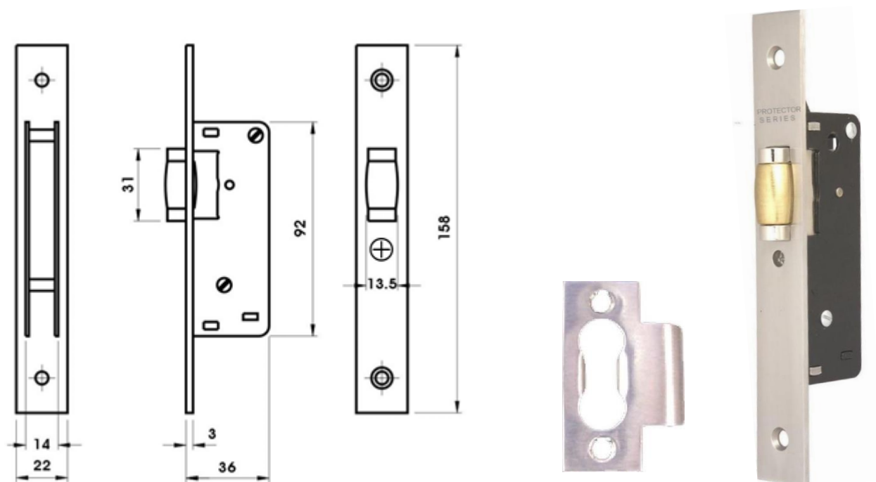
723 Strike Plate
